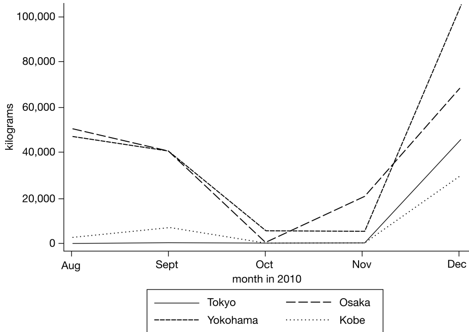
Figure 7. Yttrium Oxide
