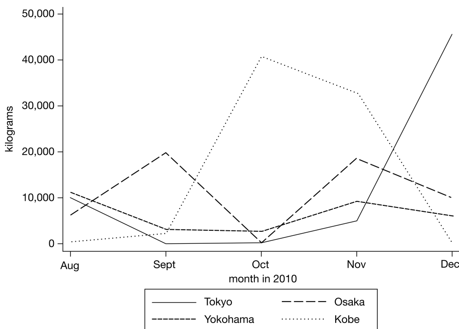
Figure 5. Cerium Oxides
